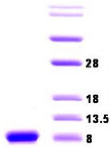
15% SDS-PAGE (3ug)
