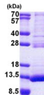
15% SDS-PAGE (3ug)
